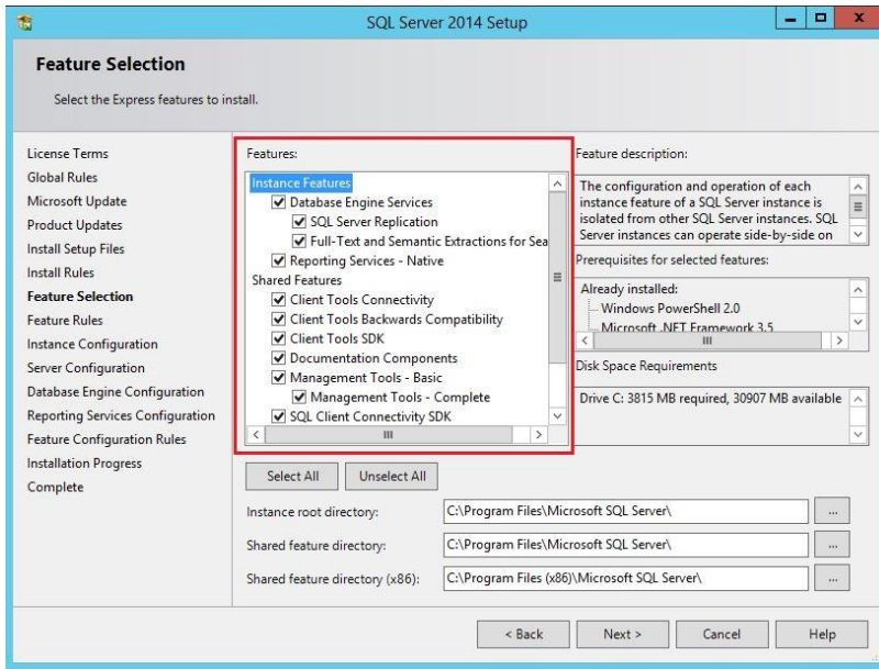
Figura 2.67 Instalación manual de SQL Express 2014 with Advanced Services
